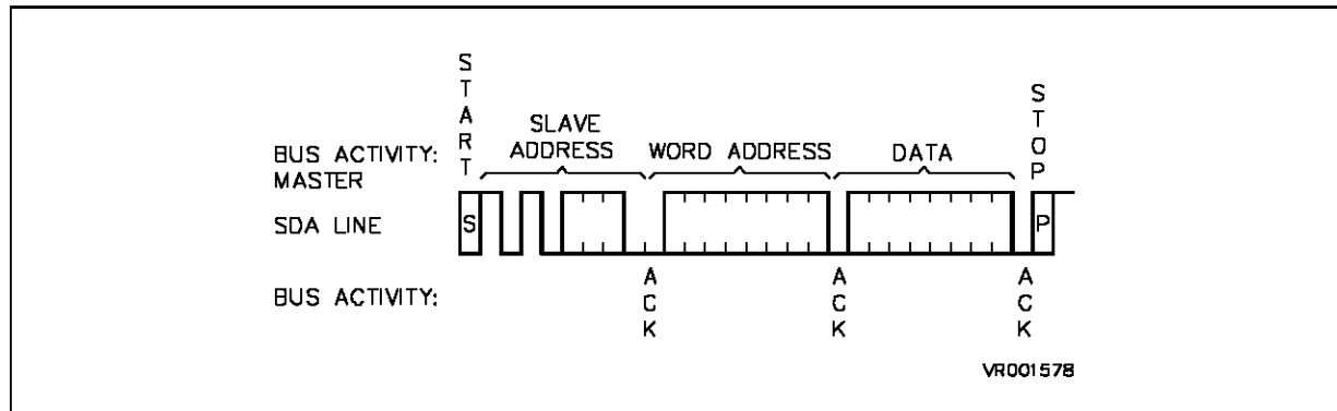
Figure 4. I 2 C-bus Protocol for Random Write Mode (1 byte)
