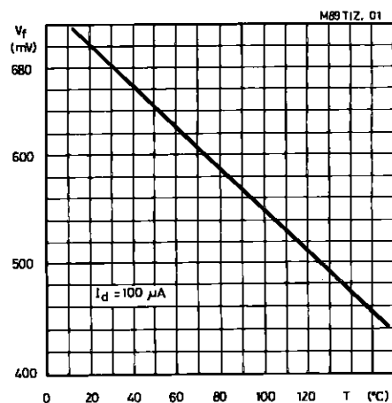
Figure A2 : Calibration Curve (sensing diode).
