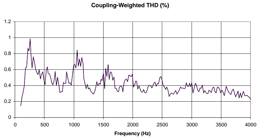
Figure 14. Coupling-Weighted THD+N
