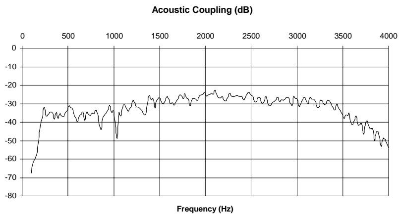
Figure 12. Example Acoustic Coupling Frequency Response
