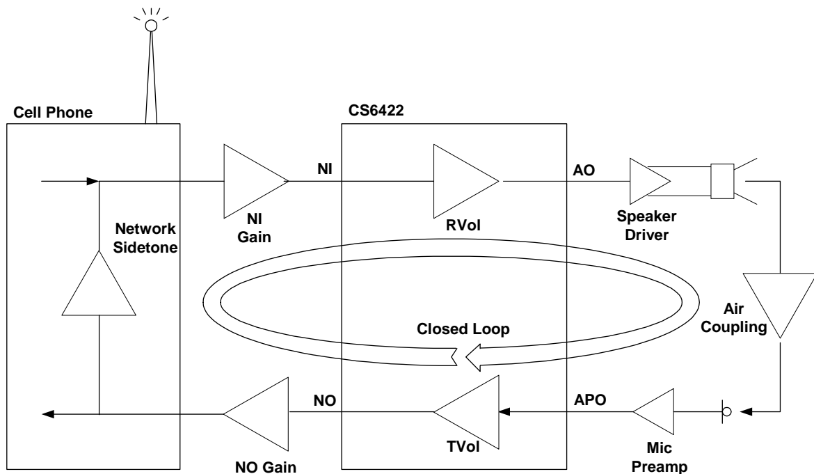
Figure 9. Loop Gain with Network Sidetone
