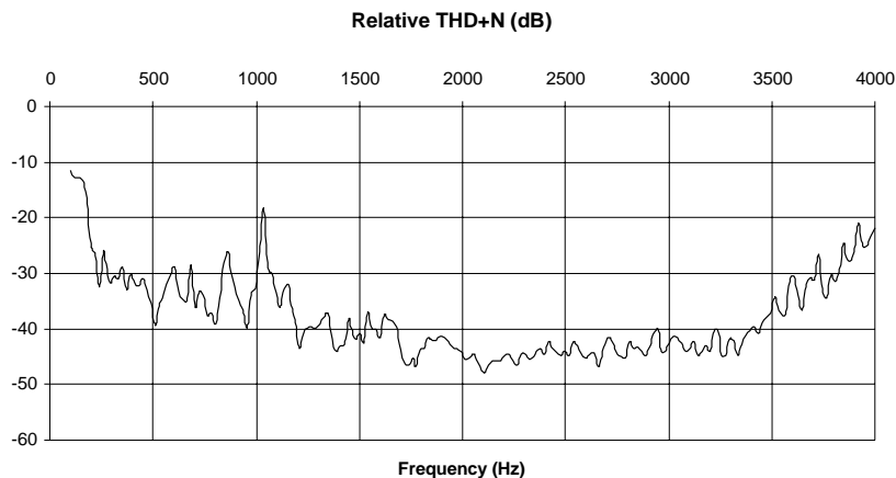
Figure 13. Relative THD+N
