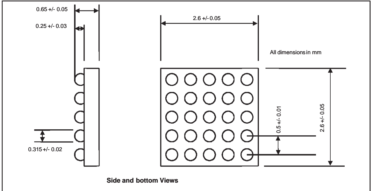
Figure 1 : Mechanical dimension of a 300µm flip chip CSP (example)
