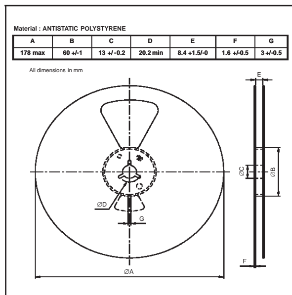
Figure 4 : 7" reel mechanical dimensions
