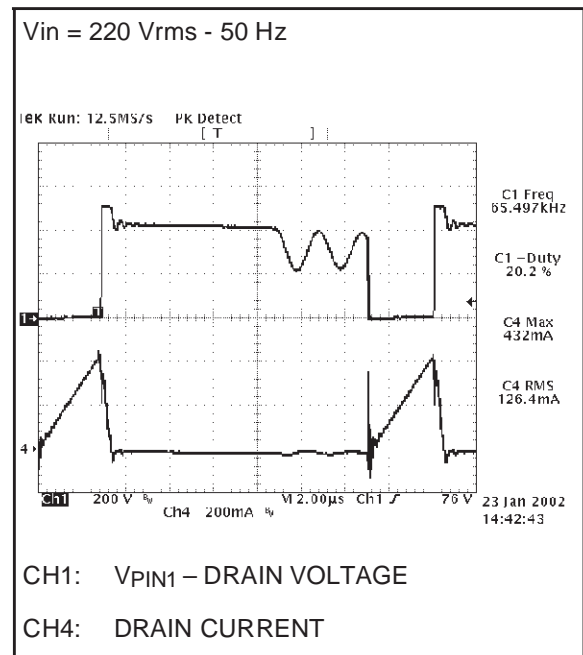
Figure 2. Vds & Id @FULL LOAD
