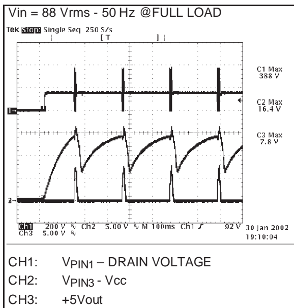
Figure 30. OPEN LOOP
