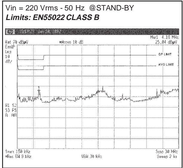
Figure 36. QUASI-PEAK MEASURE
