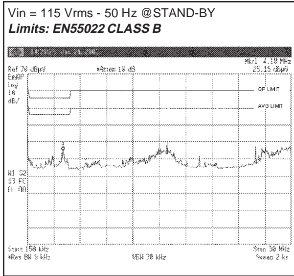
Figure 35. QUASI-PEAK MEASURE
