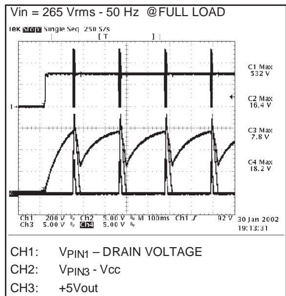
Figure 31. OPEN LOOP
