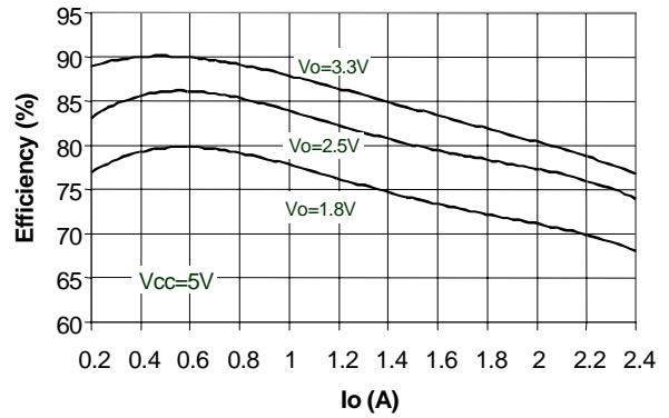
Figure 20. Efficiency vs. Output Current ( V_{CC} = 5V )
