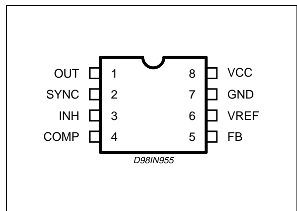
Figure 3. Pins connection
