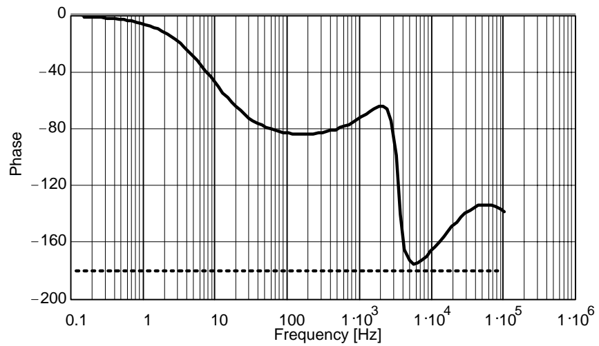
Figure 12. Phase Plot
