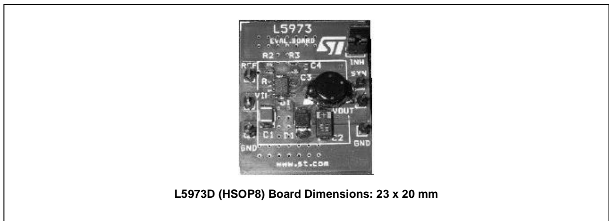
Figure 1. Demoboard
