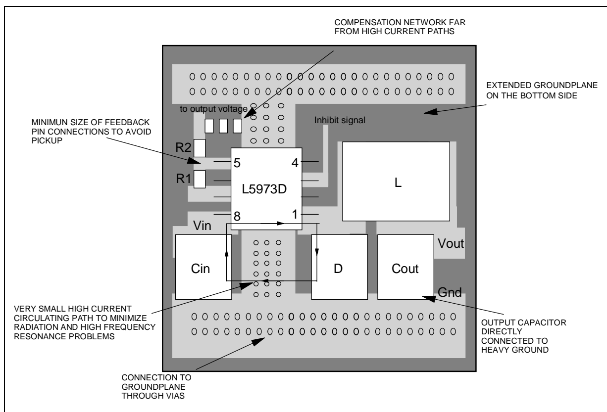
Figure 13. Layout example
