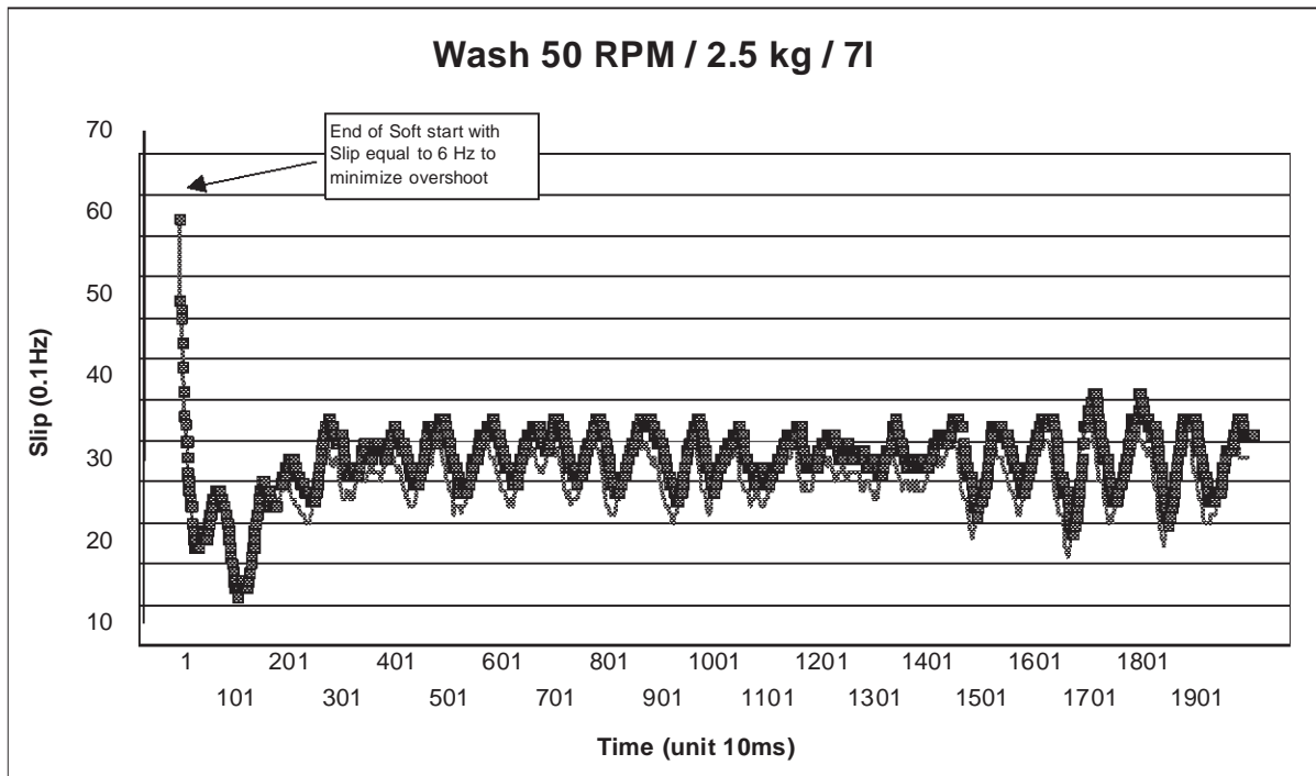
Figure 2. Slip control during washing
