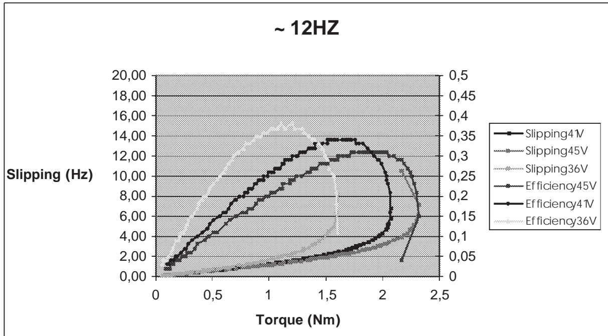
Figure 1. Induction Motor Torque versus Slip Characteristics
