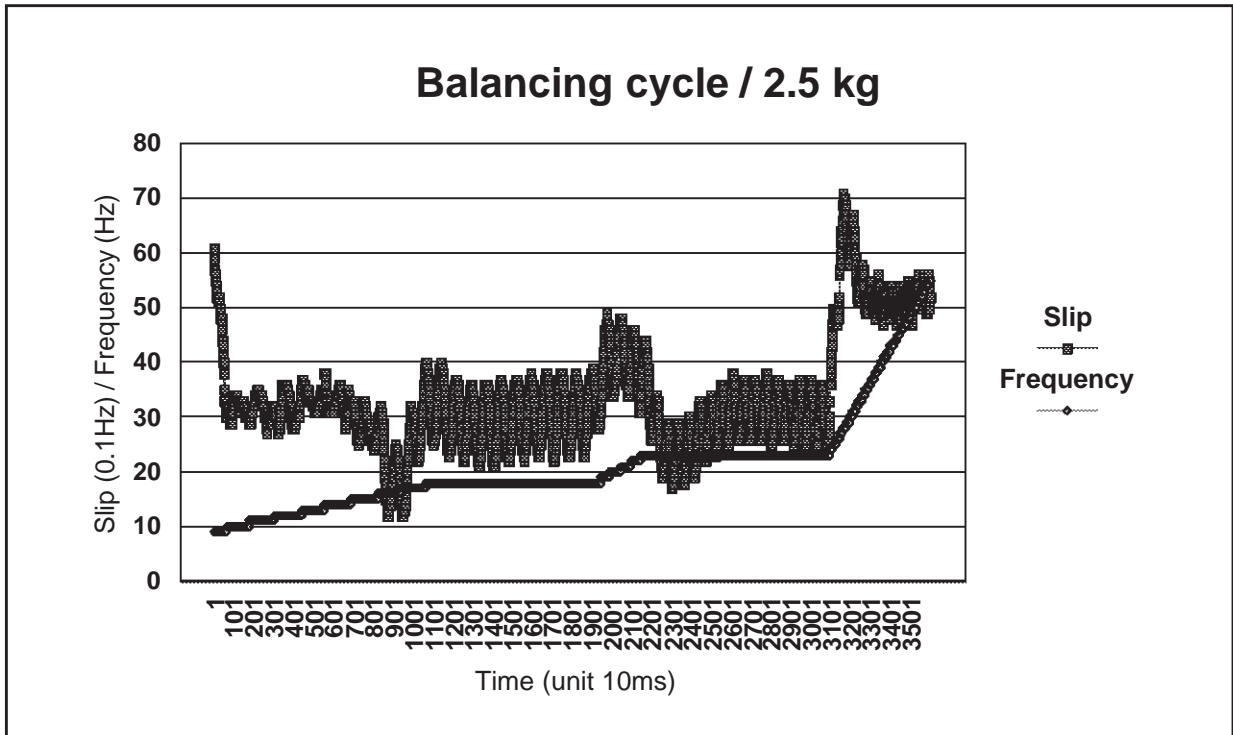
Figure 3. Slip control during balancing ramp
