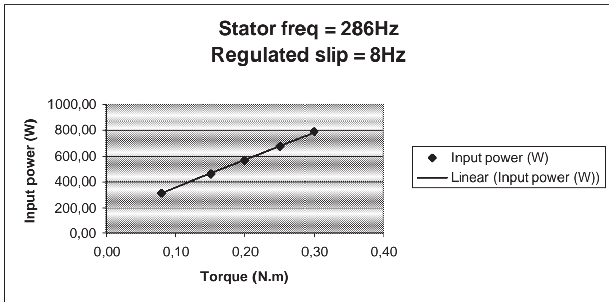
Figure 5. Power control linearity
