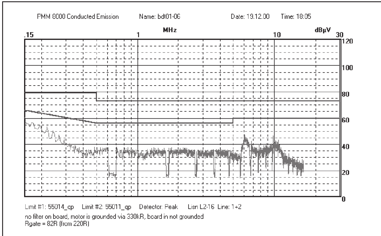
Figure 6. Conducted noise with optimum Gate drive impedance
