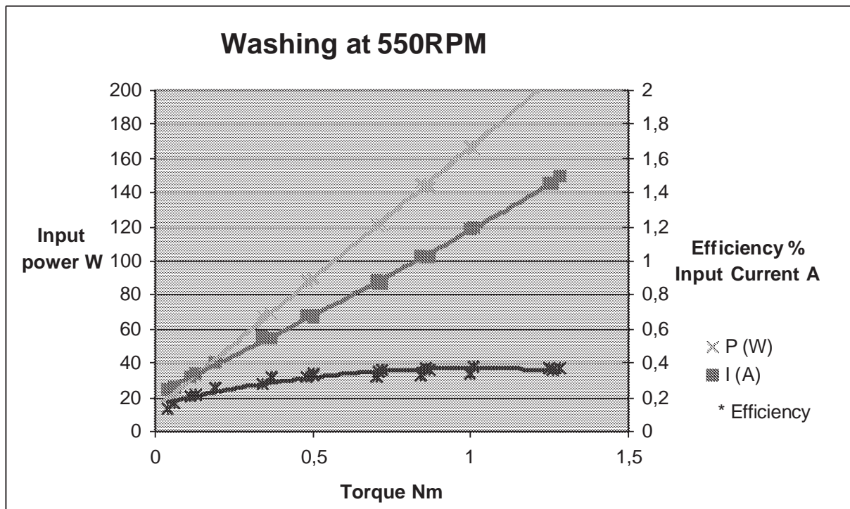
Figure 4. System (motor + drive) efficiency at very low speed (550 r.p.m. rotor)
