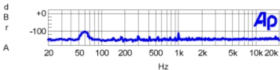
Audio Precision XICOR X9408 Separation Test Chan 0 to 2
