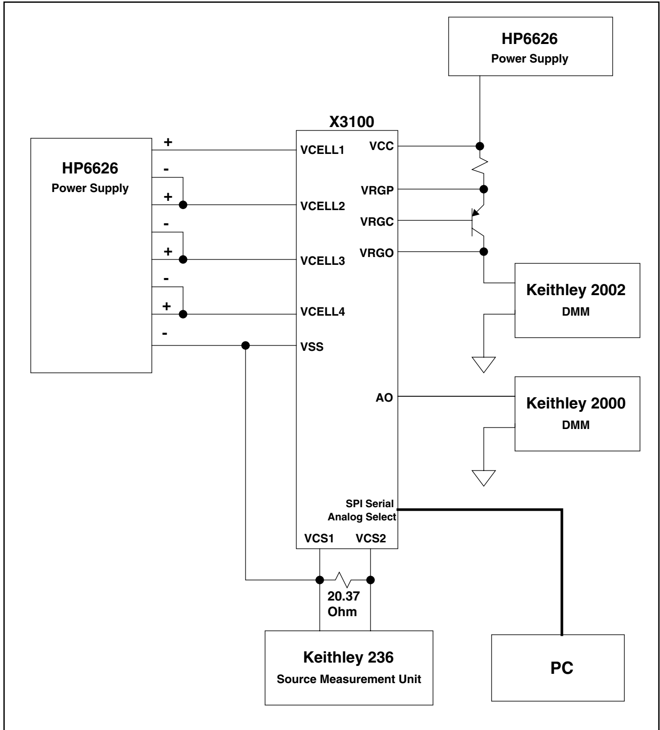
Figure 2. Characterization Test Setup
