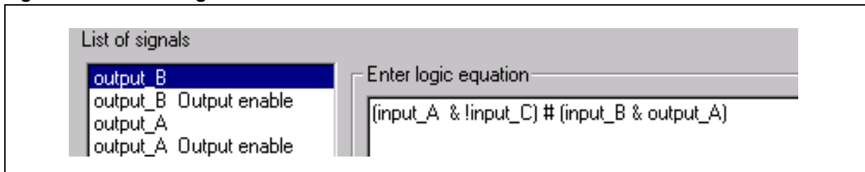
Figure 21. Generic Logic Statement
