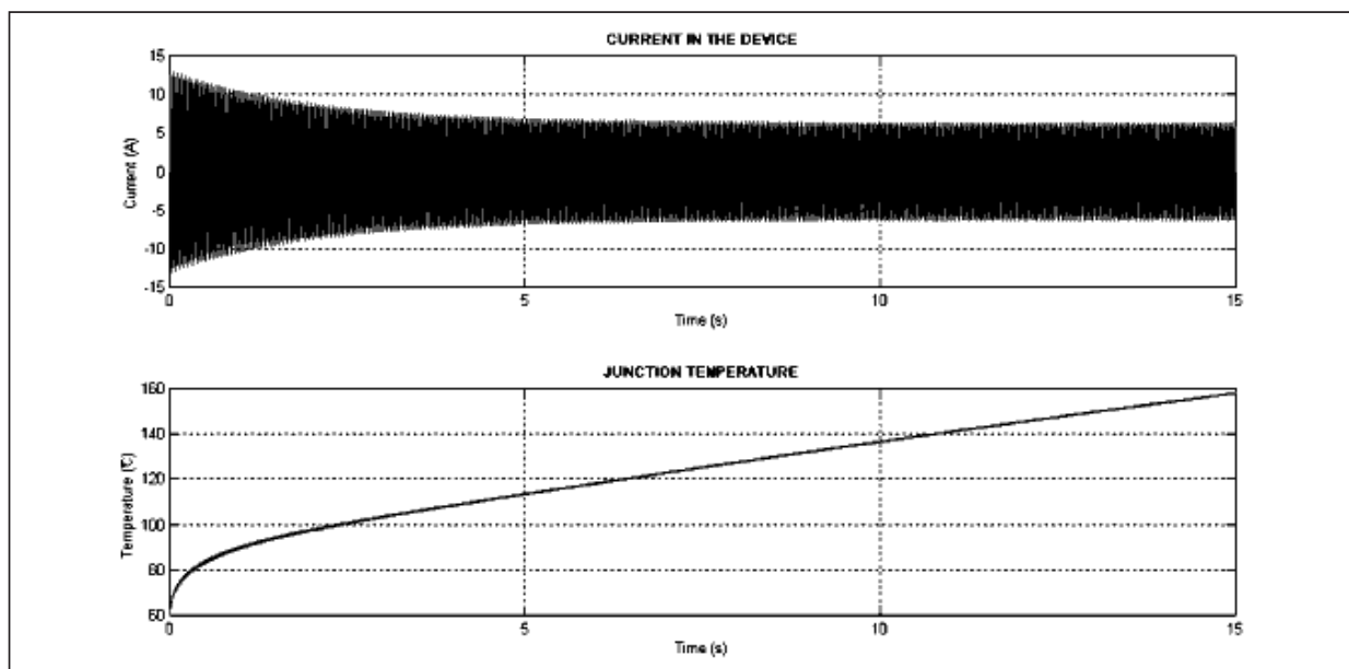
Fig. 7: Triac junction temperature during stalled rotor operation
