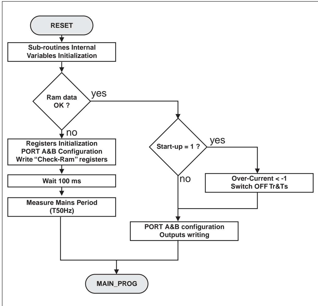
Fig. 5: Start-up procedure
