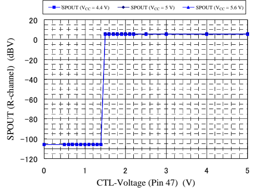
HP_JACK on/off
