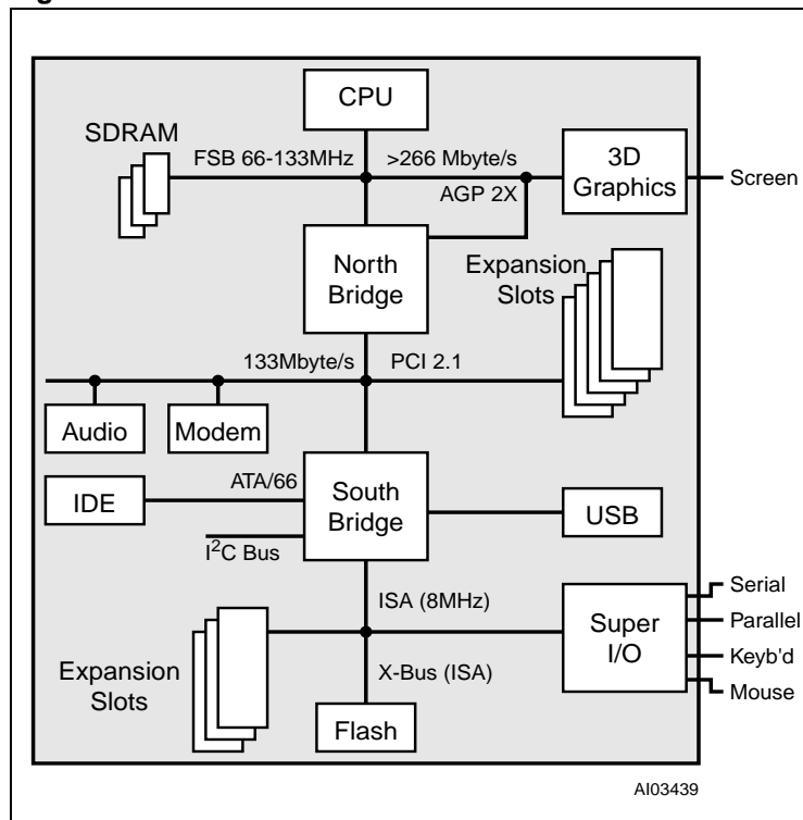
Figure 1. Earlier PC Architecture with ISA/X-bus
