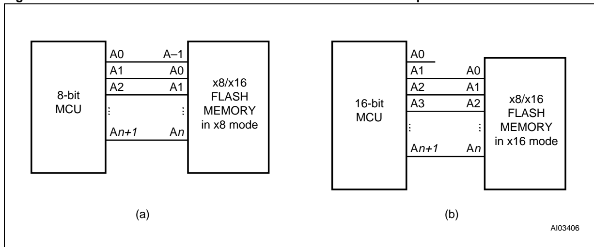
Figure 6. Connection between x8/x16 bit Flash Memories and microprocessors
