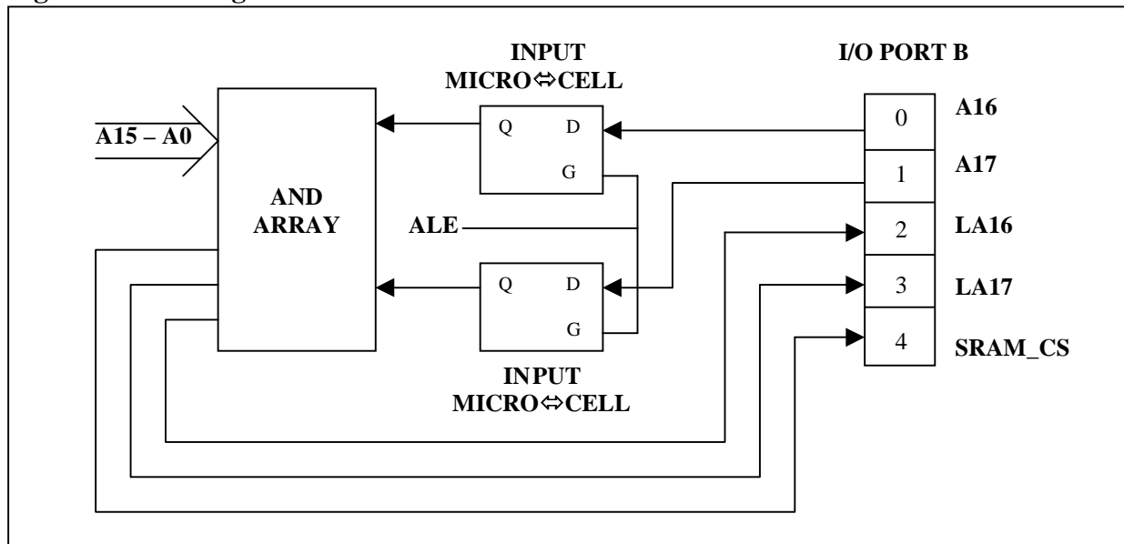
Figure 6. Latching A16 and A17 in the PSD813F5 CPLD
