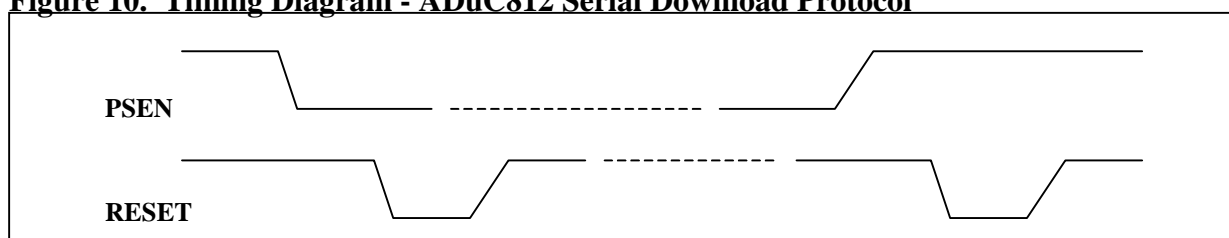
Figure 10. Timing Diagram - ADuC812 Serial Download Protocol
