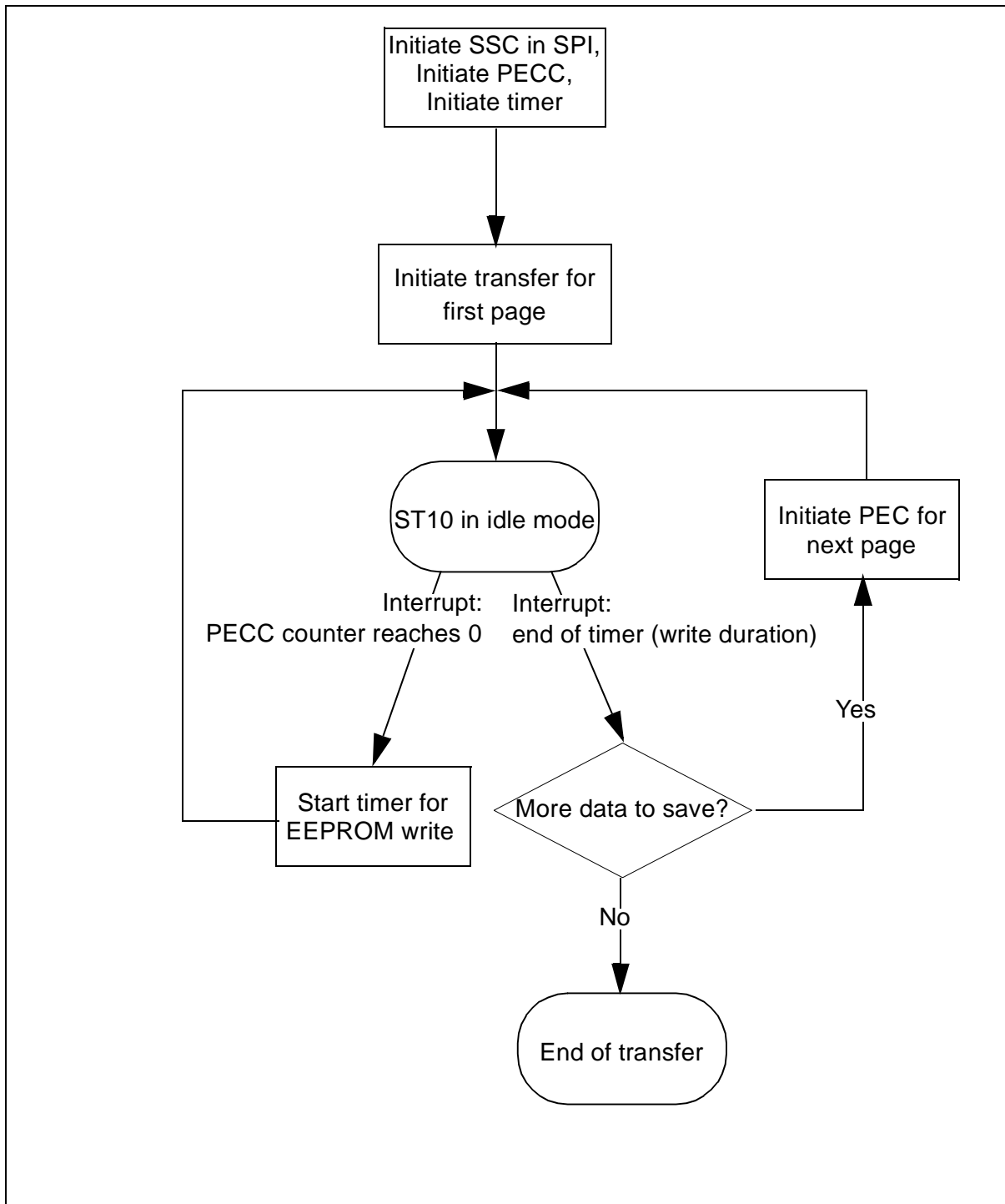
Figure 1 Program flow
