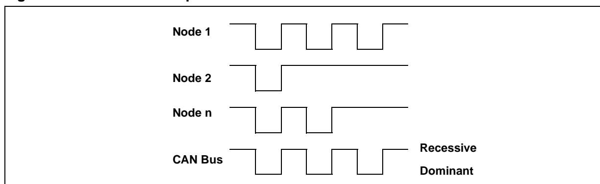
Figure 7. Arbitration example: node 1 wins
