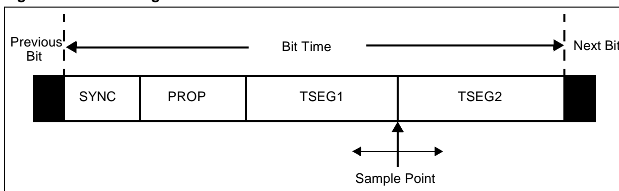
Figure 6. CAN Bit Segments
