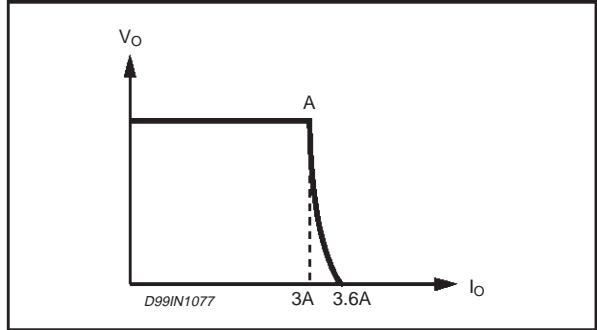
Figure 7.2. Output Characteristic
