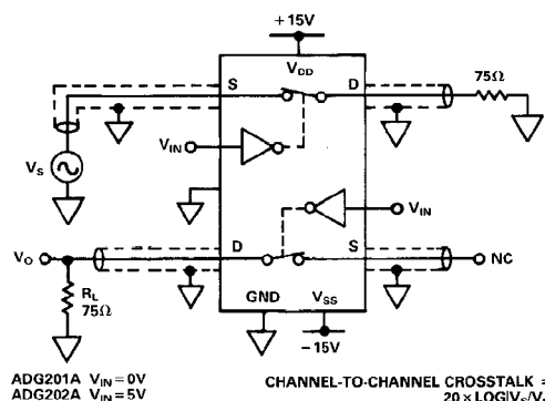
Test Circuit 7. Channel-to-Channel Crosstalk
