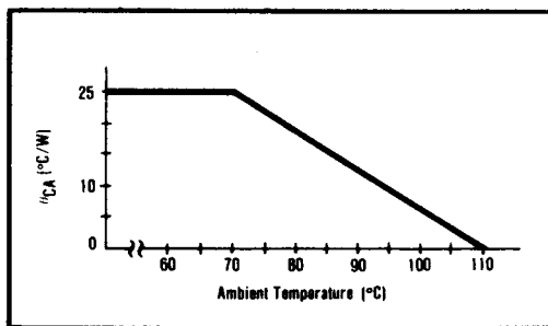
FIGURE 8. \theta_{CA} Requirement Above 70°C.
