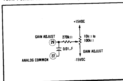
FIGURE 7. Connecting Optional Gain Adjust with a 0.2% Range of Adjustment.
