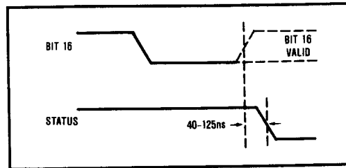
FIGURE 2b. Timing Relationship of Valid Data to Status.
