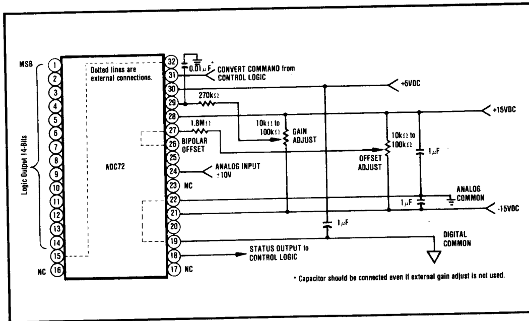
FIGURE 3. ADC72 Connections For: \pm 10V Analog Input, 14-Bit Resolution (Short-Cycled), Parallel Data Output.
