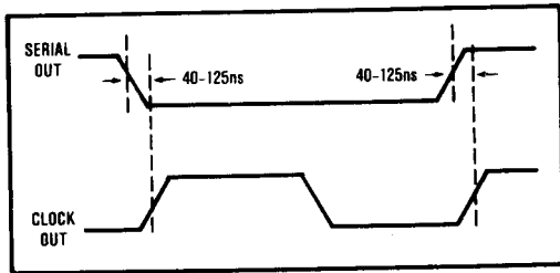
FIGURE 2a. Timing Relationship of Serial Data to Clock.
