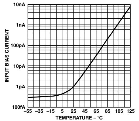
TPC 15. Pin 2 Input Bias Current vs. Temperature
