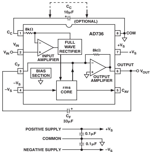
Figure 2. AD736 Average Responding Circuit
