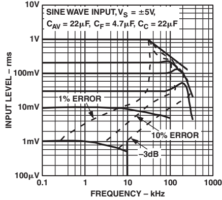
TPC 5. Frequency Response Driving Pin 2
