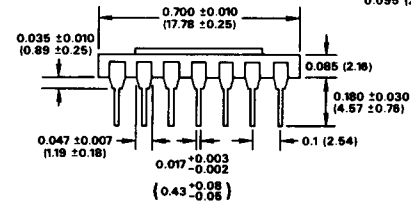
TO-116 "D" PIN CONFIGURATIONS TOP VIEW
