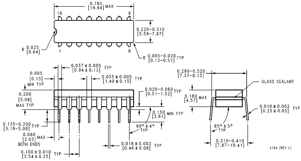
16-Lead Ceramic Dual-In-Line Package (J) Order Number 93L10DMQB or 93L16DMQB NS Package Number J16A
