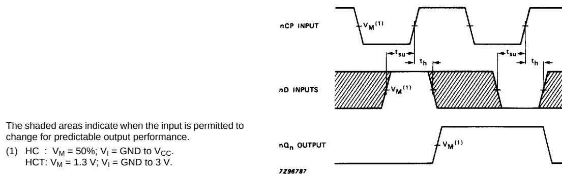
Fig.8 Waveforms showing the data set-up and hold times for nD inputs.
