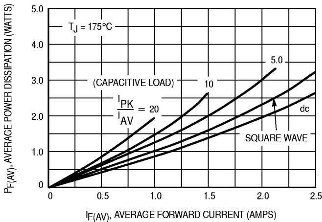
Figure 9. Power Dissipation
