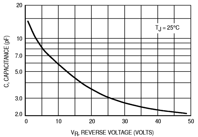
Figure 10. Typical Capacitance
