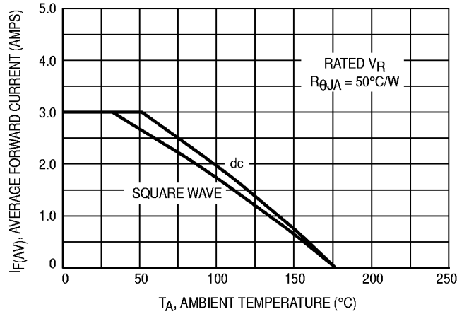
Figure 3. Current Derating (Mounting Method #3 Per Note 1)
