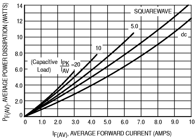
Figure 9. Power Dissipation
