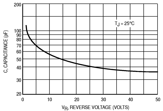
Figure 5. Typical Capacitance
