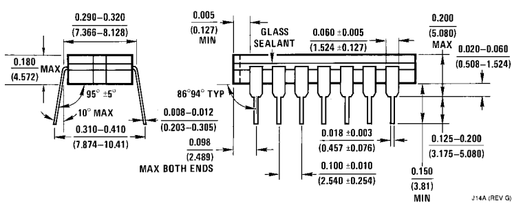
14-Lead Ceramic Dual-In-Line Package (J) Order Number 54LS14DMQB NS Package Number J14A
