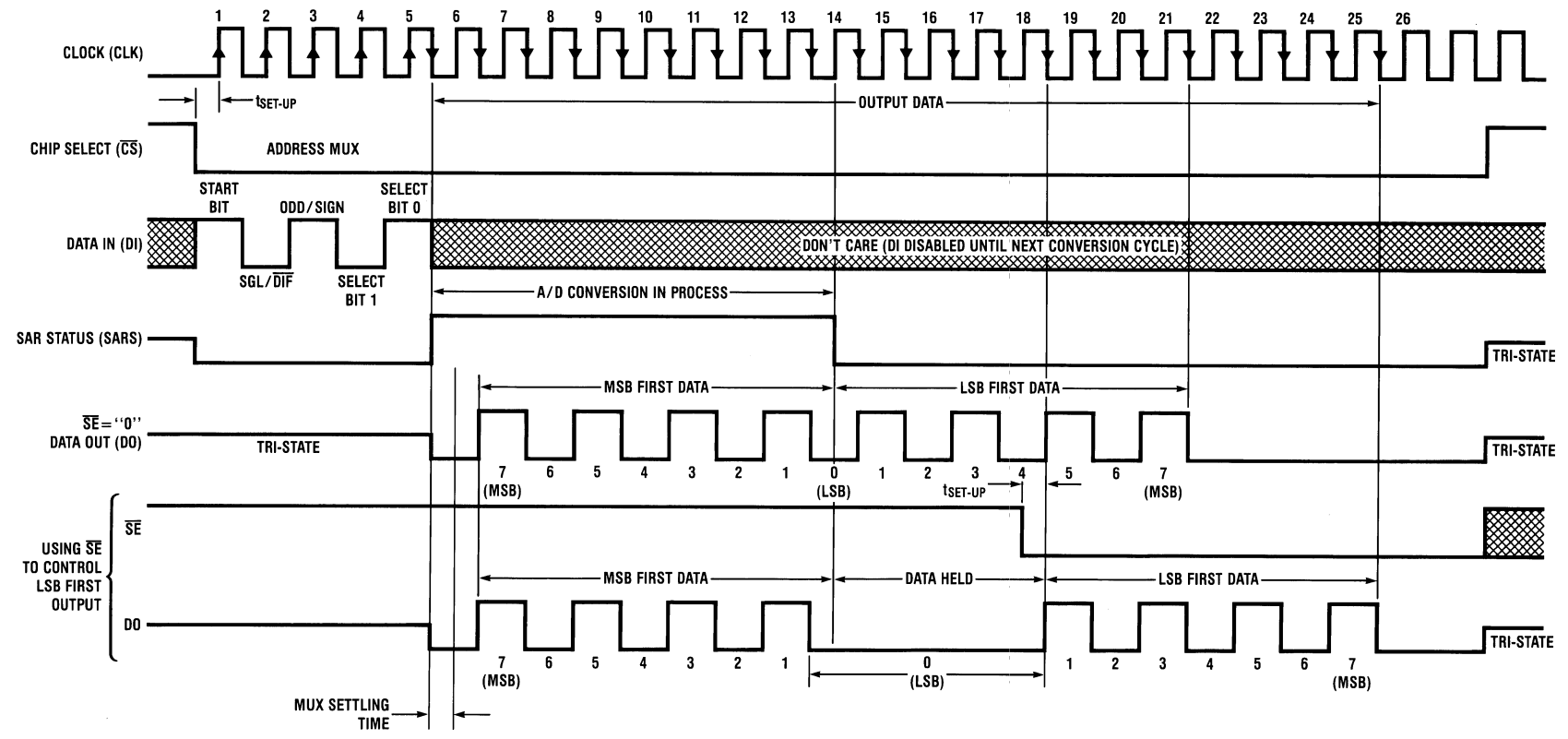
ADC0838 Timing
