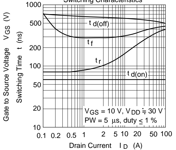
Switching Characteristics
