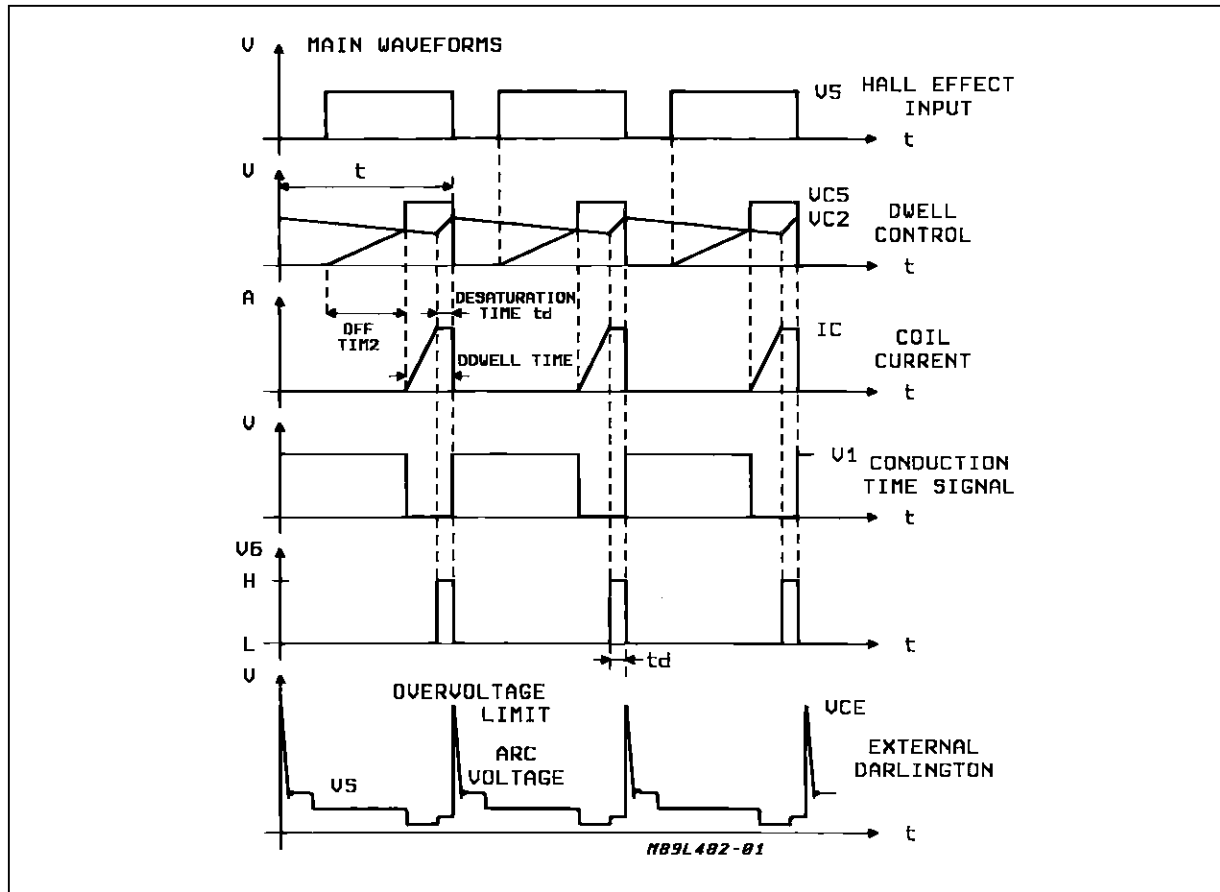
Figure 1 : Main Waveforms.
