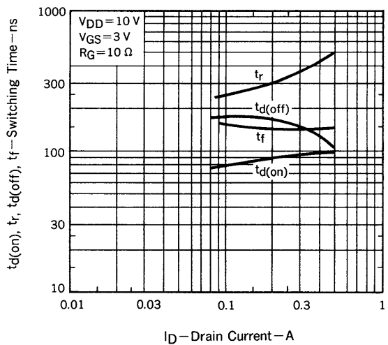
SWITCHING CHARACTERISTICS
