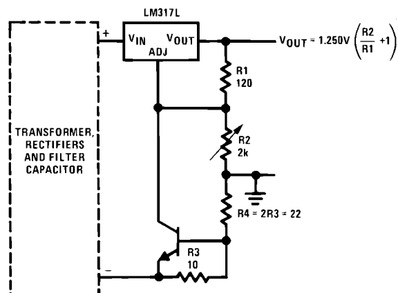
Adjustable Regulator with Current Limiter
