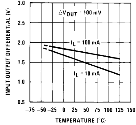
Dropout Voltage
