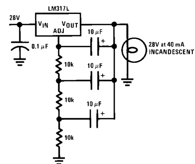
Lamp Flasher
