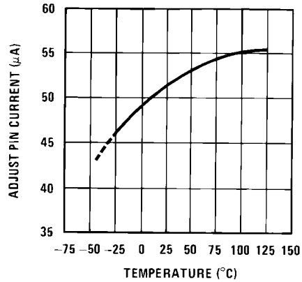
Adjustment Current
