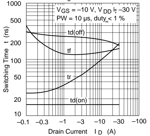
Switching Characteristics
