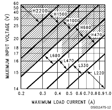
FIGURE 5. LM2575(HV)-12
