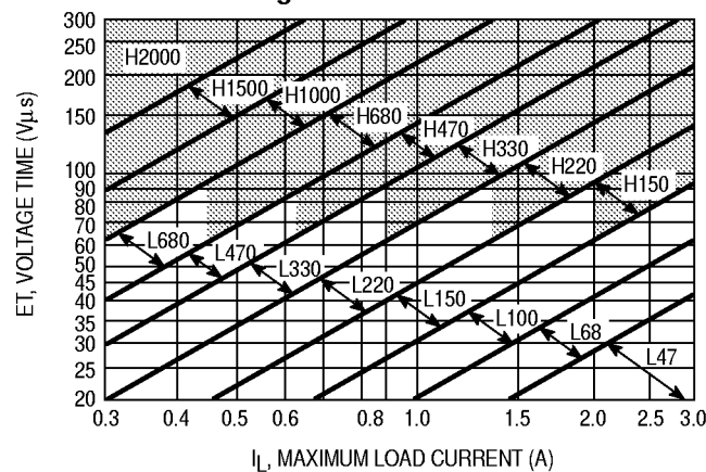
Figure 22. LM2576-ADJ
