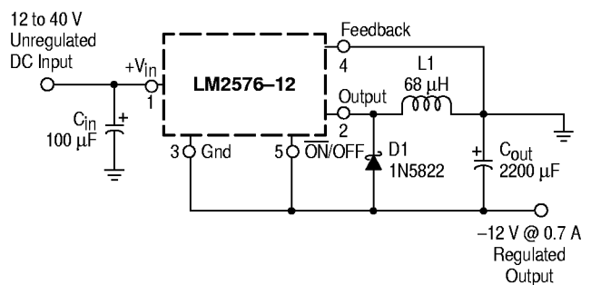
Figure 26. Inverting Buck–Boost Develops -12\text{ V}
