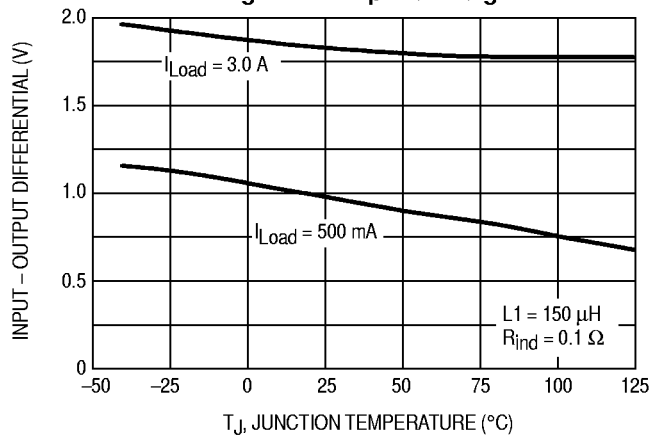
Figure 4. Dropout Voltage
