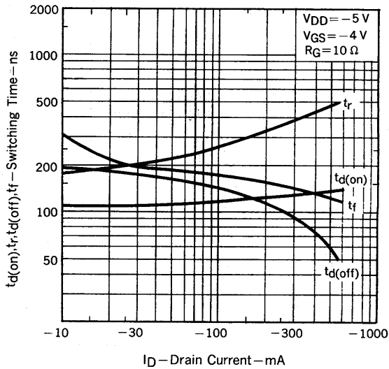
SWITCHING CHARACTERISTICS
