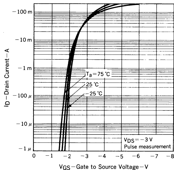
TRANSFER CHARACTERISTICS
