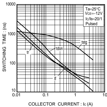
Fig.7 Switching time
