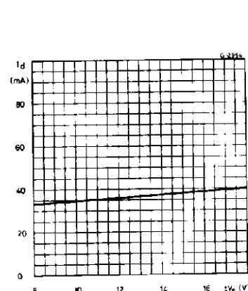
Figure 9. Quiescent current vs. supply voltage
