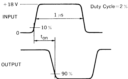
VOLTAGE WAVEFORMS
