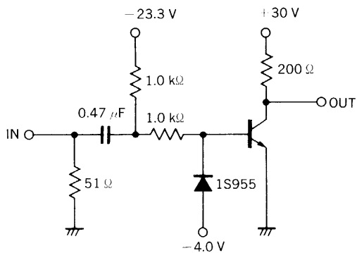
t_{off} SWITCHING
