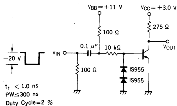
t_{off} SWITCHING
