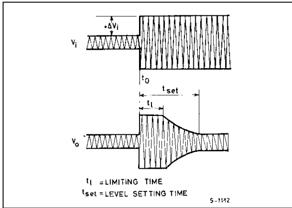
Figure 17: Limiting and Level Setting Time
