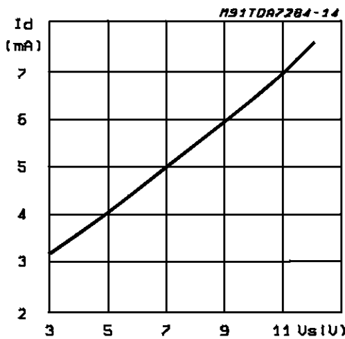
Figure 3: Drain Current vs. Supply Voltage
