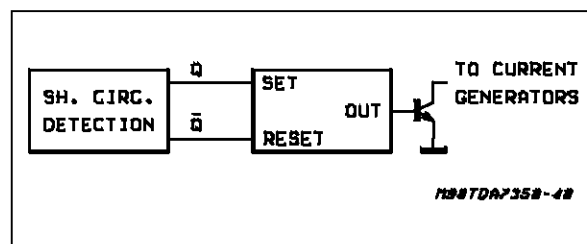
Figure 38: Restart Circuit
