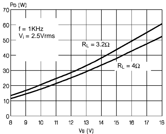
Figure 10: EIAJ Power vs. Supply Voltage
