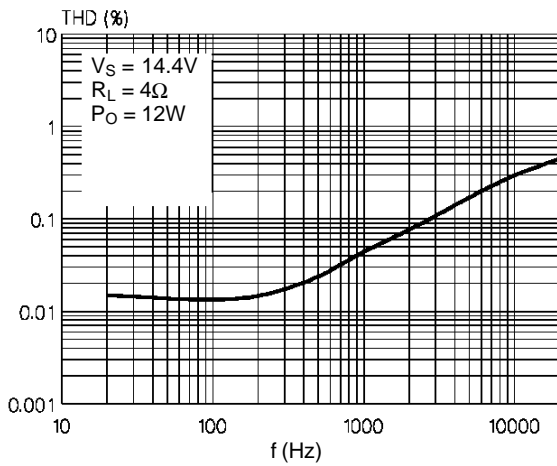
Figure 11: THD vs. Frequency
