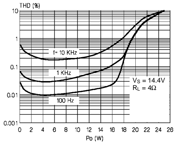
Figure 12: THD vs. Output Power
