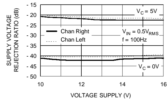
Figure 4 : Supply Voltage Rejection
