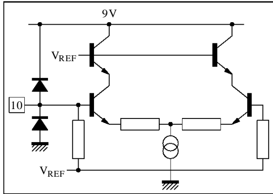
Figure 11 : Pin 10 Configuration
