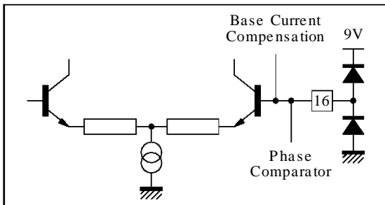
Figure 15 : Pin 16 Configuration
