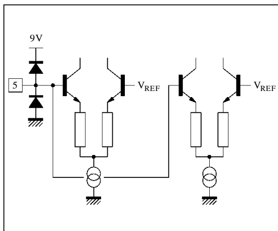
Figure 7 : Pin 5 Configuration
