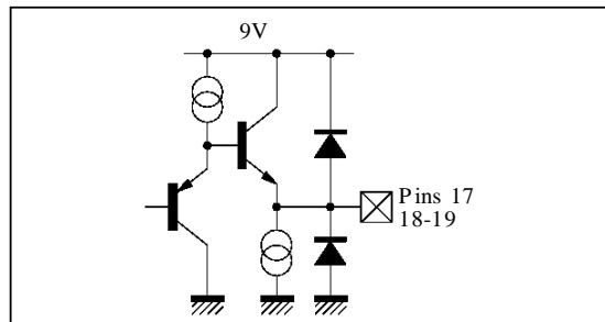
Figure 16 : Pins 17 - 18 - 19 Configuration
