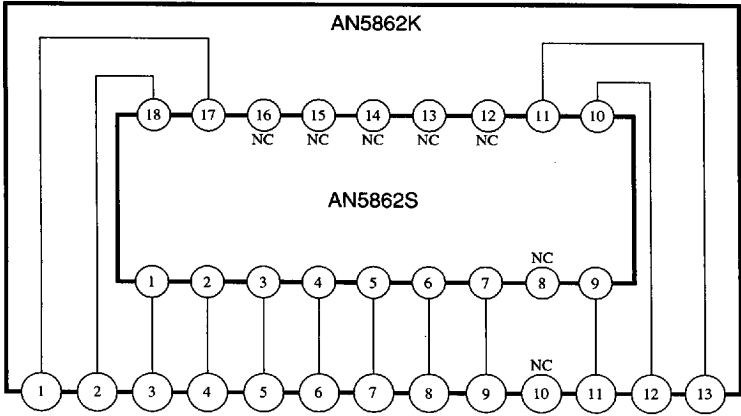
Pinning comparing table of the AN5862K and AN5862S
