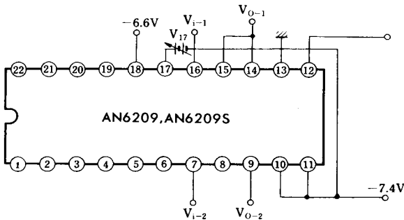
Test Circuit 17 ( V_{17-ON} )
