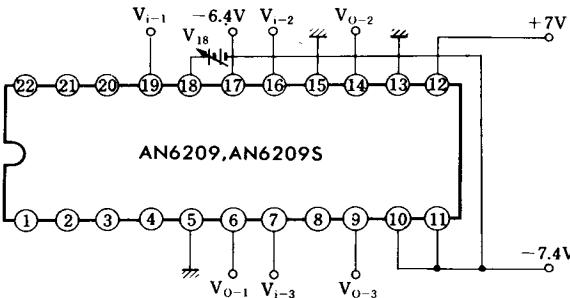
Test Circuit 15 ( V_{18-R} )
