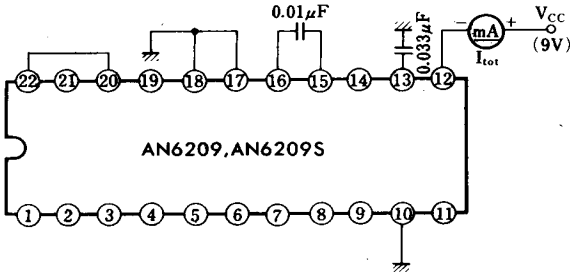
Test Circuit 13 ( I_{tot} )
