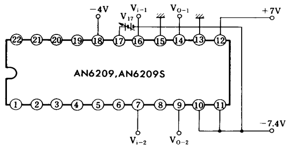
Test Circuit 16 ( V_{17-OFF} )
