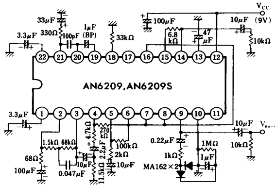
Test Circuit 9 ( V_{O(AGC1)} , V_{O(AGC2)} , THD-A)
