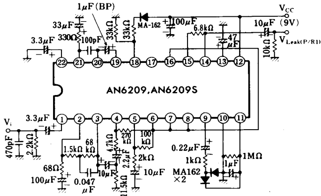
Test Circuit 11 ( V_{Leak(P/R2)} )
