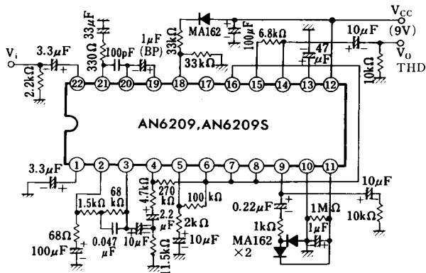
Test Circuit 9 ( V_{O(AGC1)} , V_{O(AGC2)} , THD-A)
