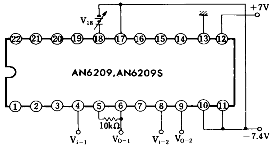
Test Circuit 14 ( V_{18-P} )
